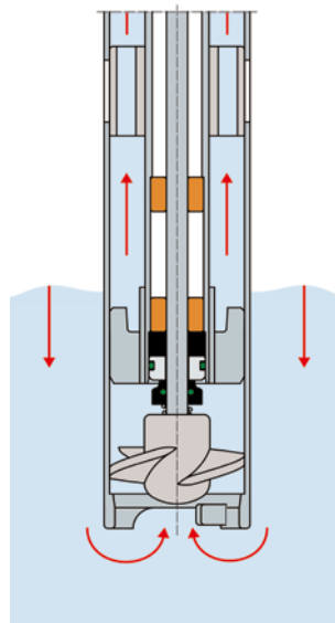
Outlet opened, mixing openings closed.
