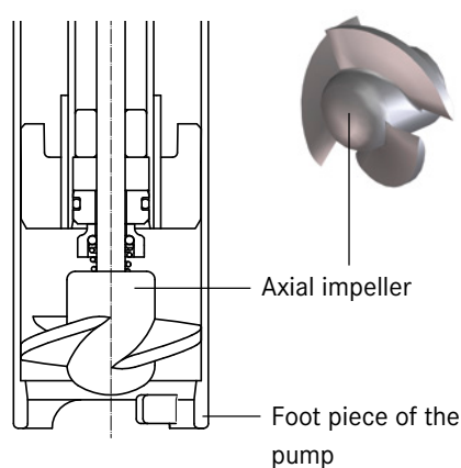
F/FP 430 with mechanical seal and axial impeller
