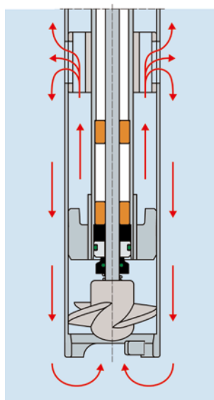
Outlet closed, mixing openings opened.
