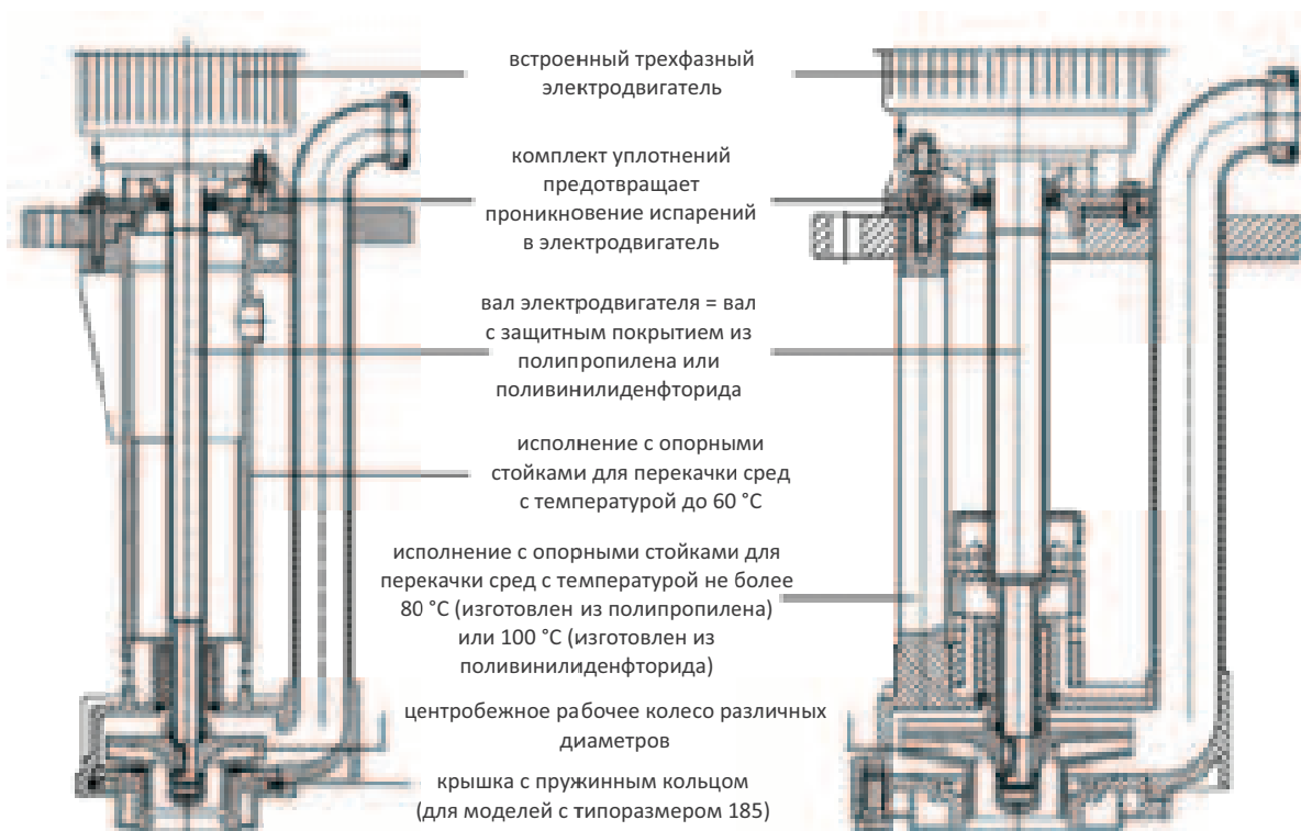
F 716 PVDF2-230
